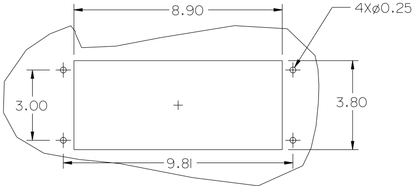
DETAIL A SCALE 0.250
